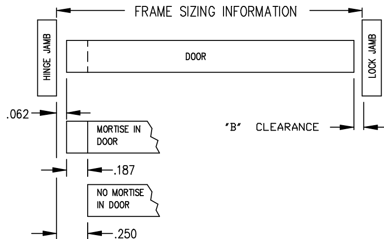
DOOR SIZES, WEIGHTS AND CLEARANCE "B"
